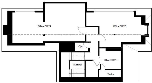
EXISTING SECOND FLOOR PLAN 1:100
